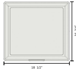
Extra Width Tote: Top View
